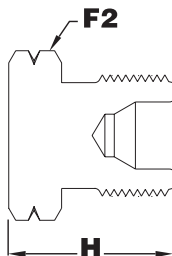
VacuSeal® Male CGA 350
