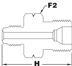
VacuSeal® Male CGA 350
